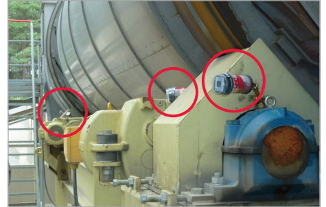
Lubrication of pillow block bearing on a rotary dryer
