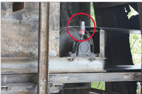
Lubrication of shaft bearing on a conveyor belt drum
