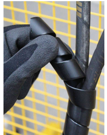
Apply spiral wrap to hoses to protect them from rubbing and to reduce catch hazards
